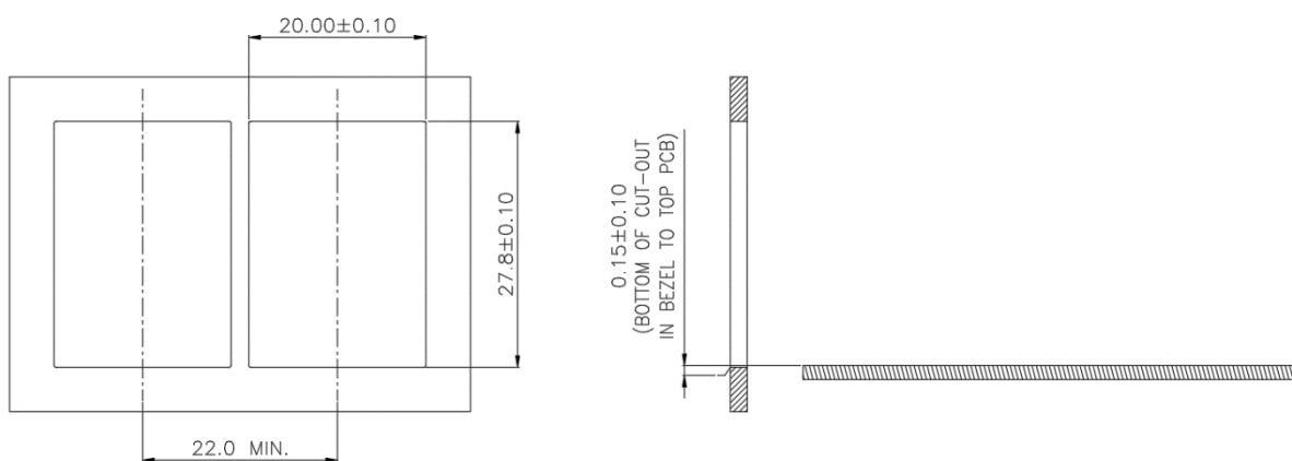
Figure 21 QSFP112 2X1 SMT and Qpath112 Bezel opening
