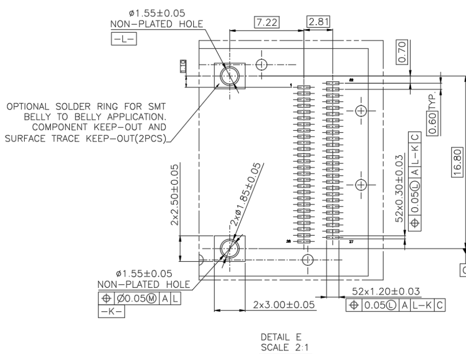
Figure 16 QSFP112 1x1 SMT Connector and cage PCB layout, Detail E
