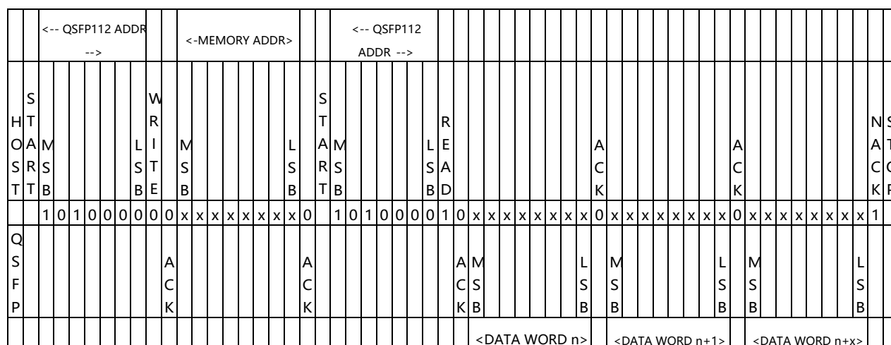
Figure 44 Sequential address read starting with random QSP112 read
